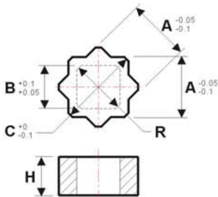
11M9 to 22M19 DESIGN
