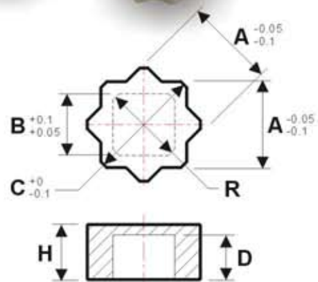
27M14 to 36M27 DESIGN
